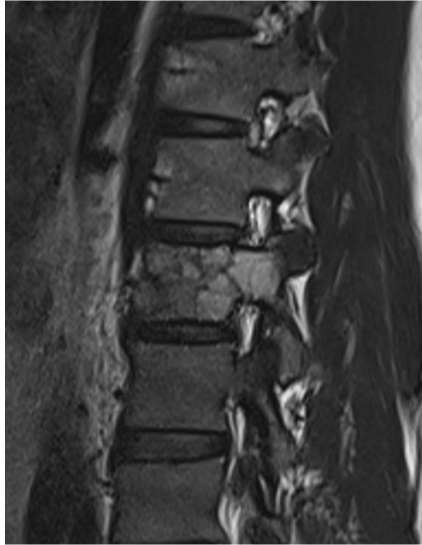
T2WI
