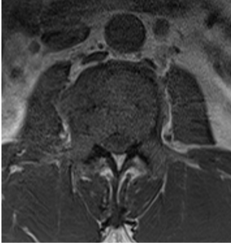
T1WI
