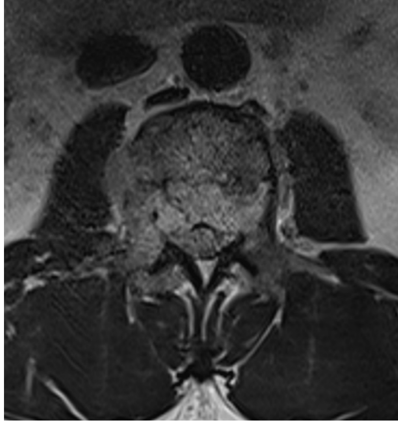
T2WI
