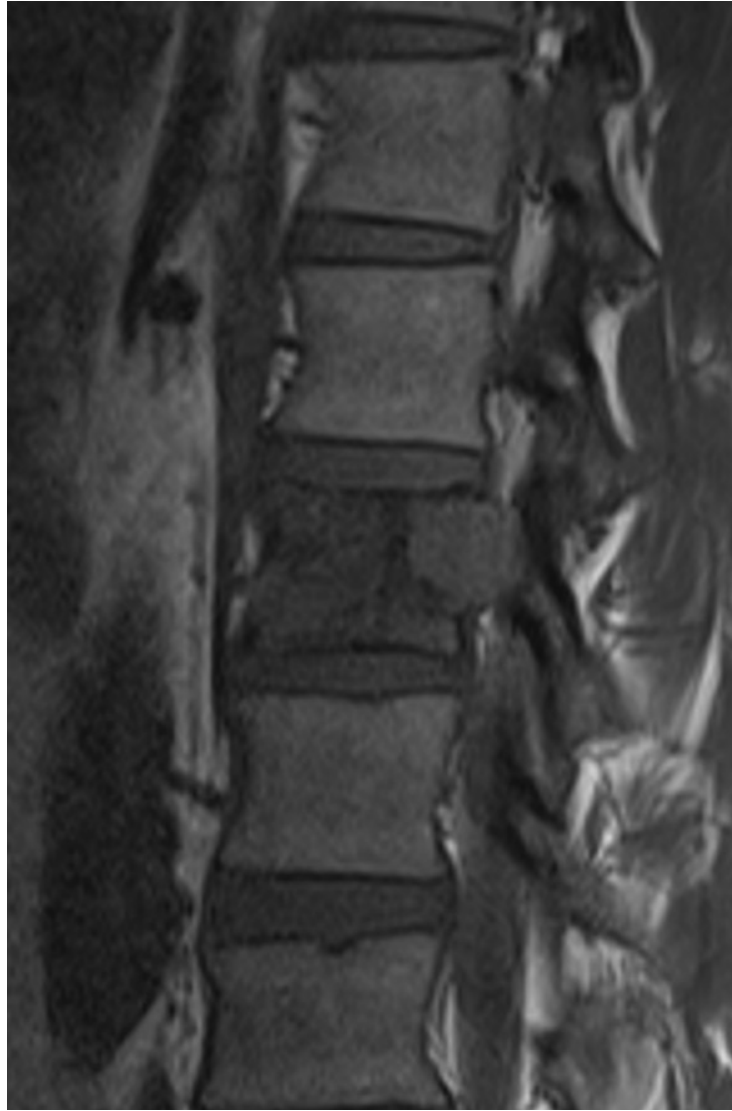
T1WI
